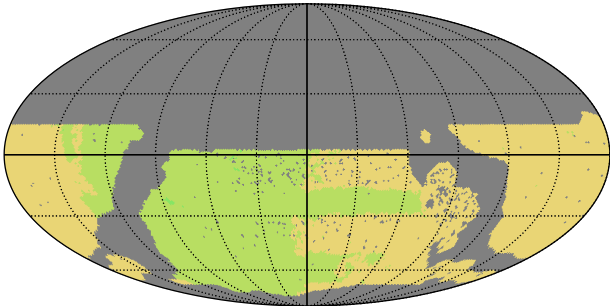
too_elab_r32_d2_griz_v3.4_10yrs WFD all bands: NSeasons
