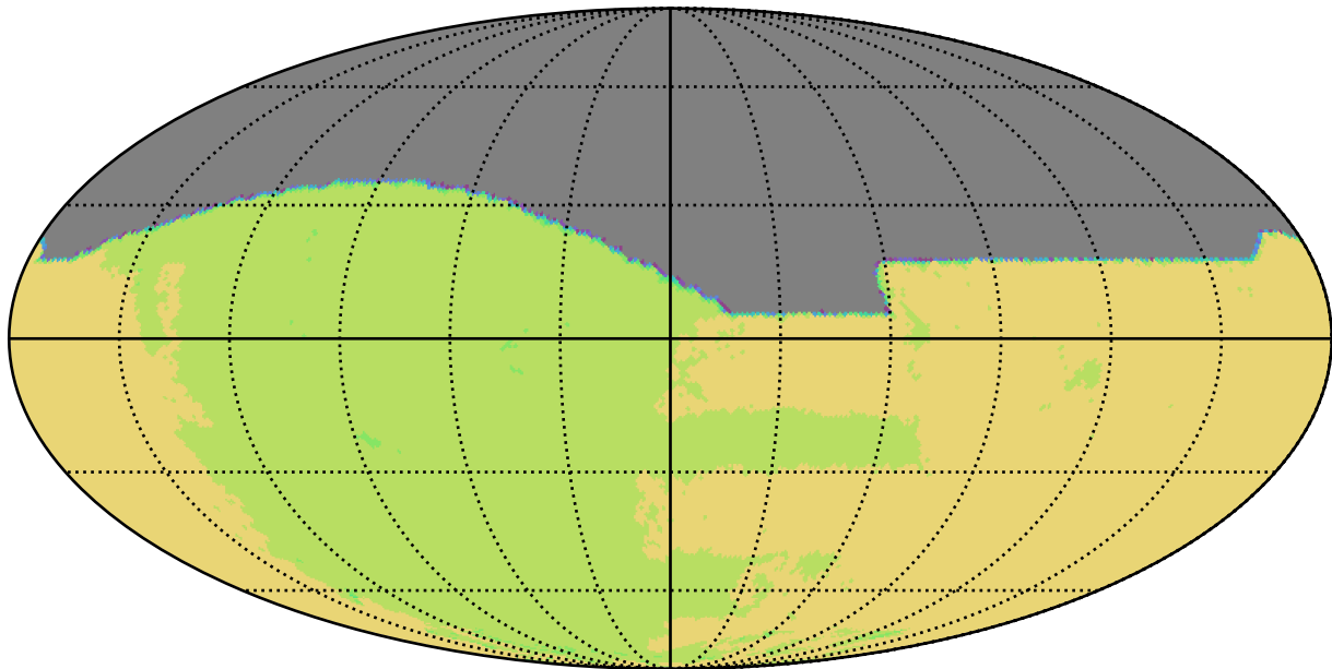
too_elab_r32_d2_griz_v3.4_10yrs All sky all bands: NSeasons
