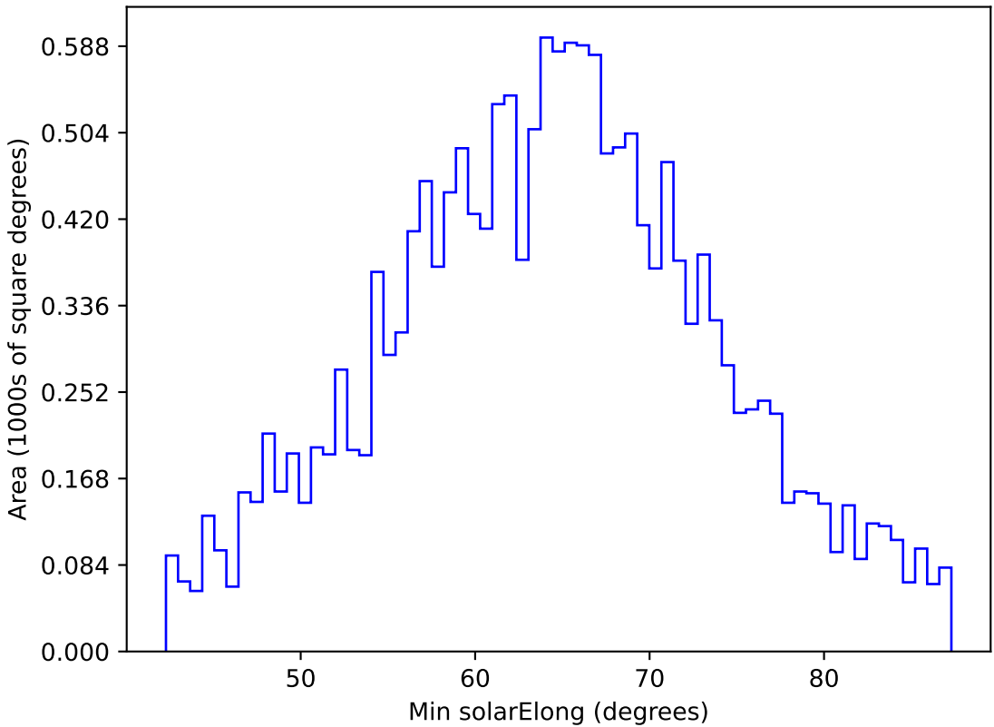
too_elab_r32_d2_griz_v3.4_10yrs WFD y band: Min solarElong
