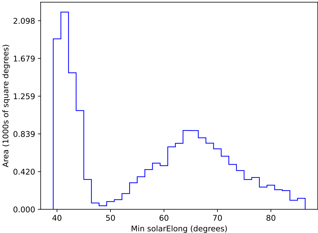
too_elab_r32_d2_griz_v3.4_10yrs WFD r band: Min solarElong
