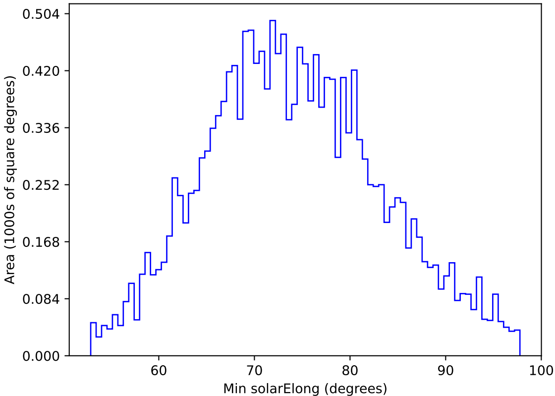
too_elab_r32_d2_griz_v3.4_10yrs WFD g band: Min solarElong
