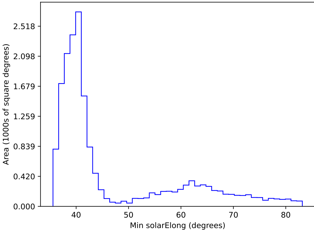
too_elab_r32_d2_griz_v3.4_10yrs WFD all bands: Min solarElong
