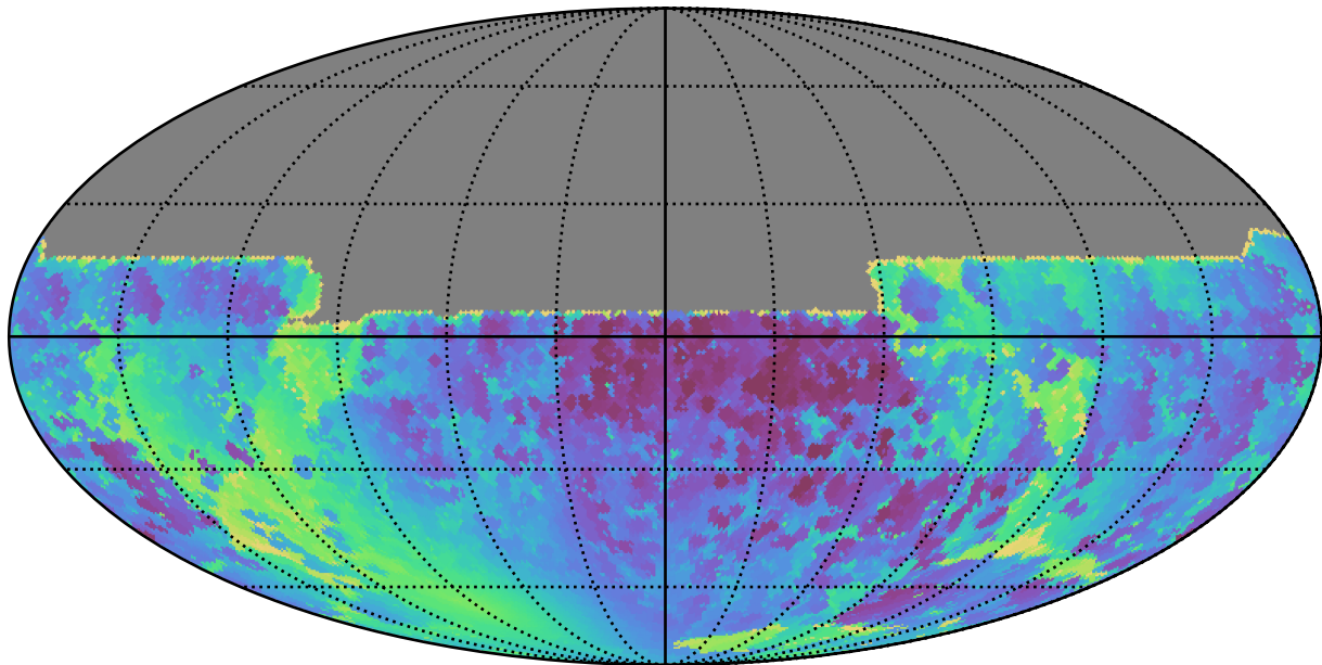
too_elab_r32_d2_griz_v3.4_10yrs All sky y band: Min solarElong
