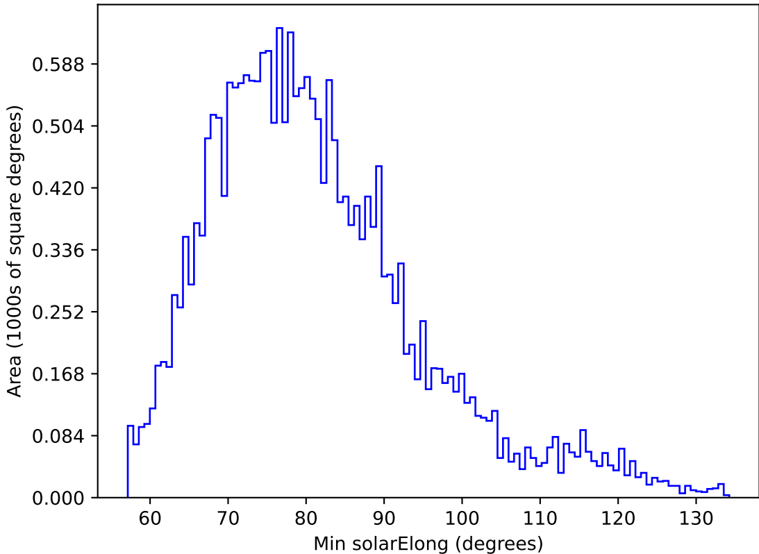
too_elab_r32_d2_griz_v3.4_10yrs All sky u band: Min solarElong
