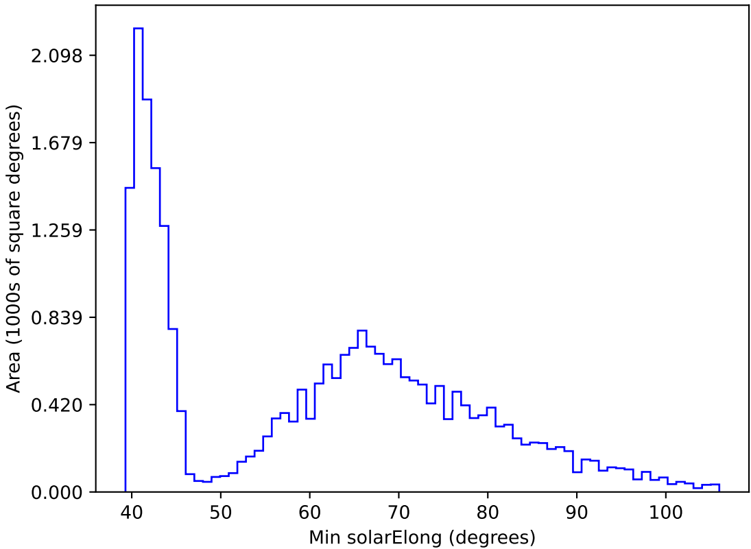
too_elab_r32_d2_griz_v3.4_10yrs All sky r band: Min solarElong
