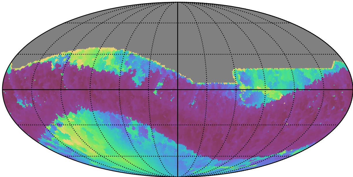
too_elab_r32_d2_griz_v3.4_10yrs All sky i band: Min solarElong
