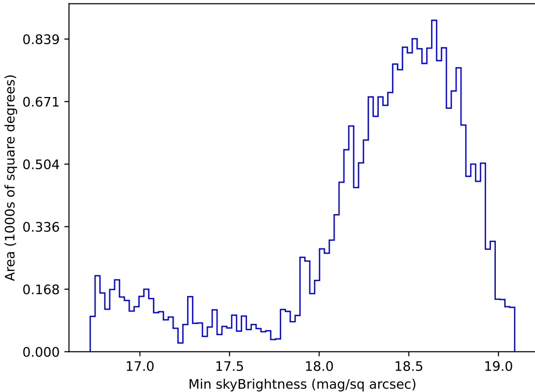
too_elab_r32_d2_griz_v3.4_10yrs Yr 1 z band: Min skyBrightness
