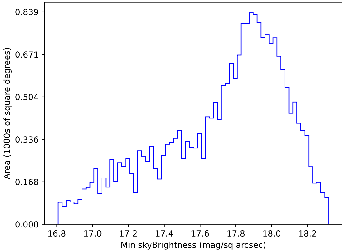
too_elab_r32_d2_griz_v3.4_10yrs Yr 1 y band: Min skyBrightness
