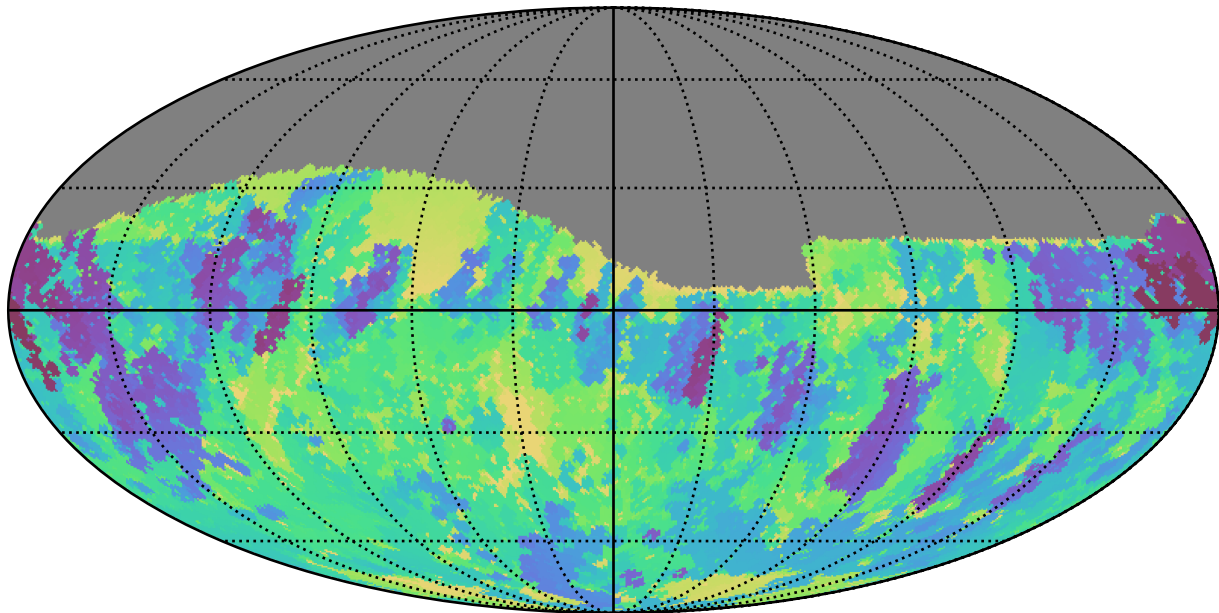
too_elab_r32_d2_griz_v3.4_10yrs Yr 1 r band: Min skyBrightness
