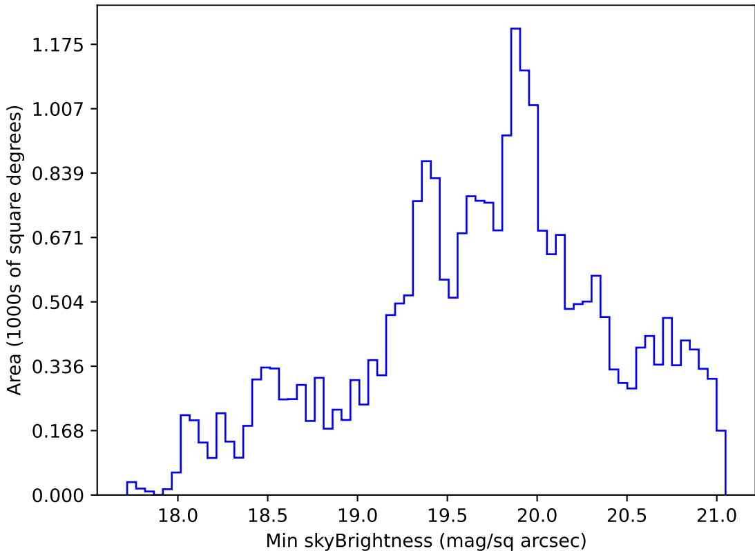
too_elab_r32_d2_griz_v3.4_10yrs Yr 1 r band: Min skyBrightness
