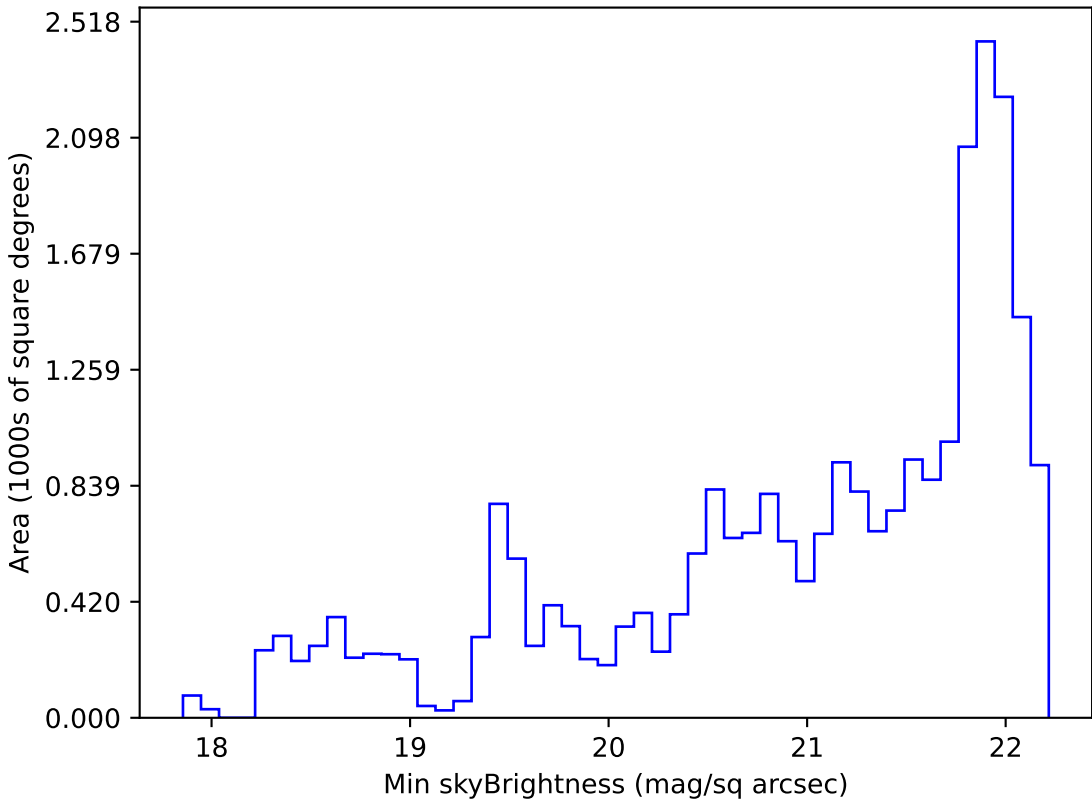
too_elab_r32_d2_griz_v3.4_10yrs Yr 1 g band: Min skyBrightness
