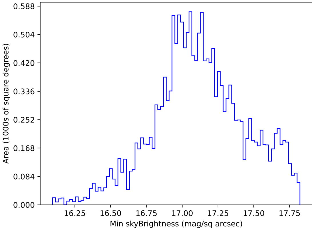
too_elab_r32_d2_griz_v3.4_10yrs WFD y band: Min skyBrightness
