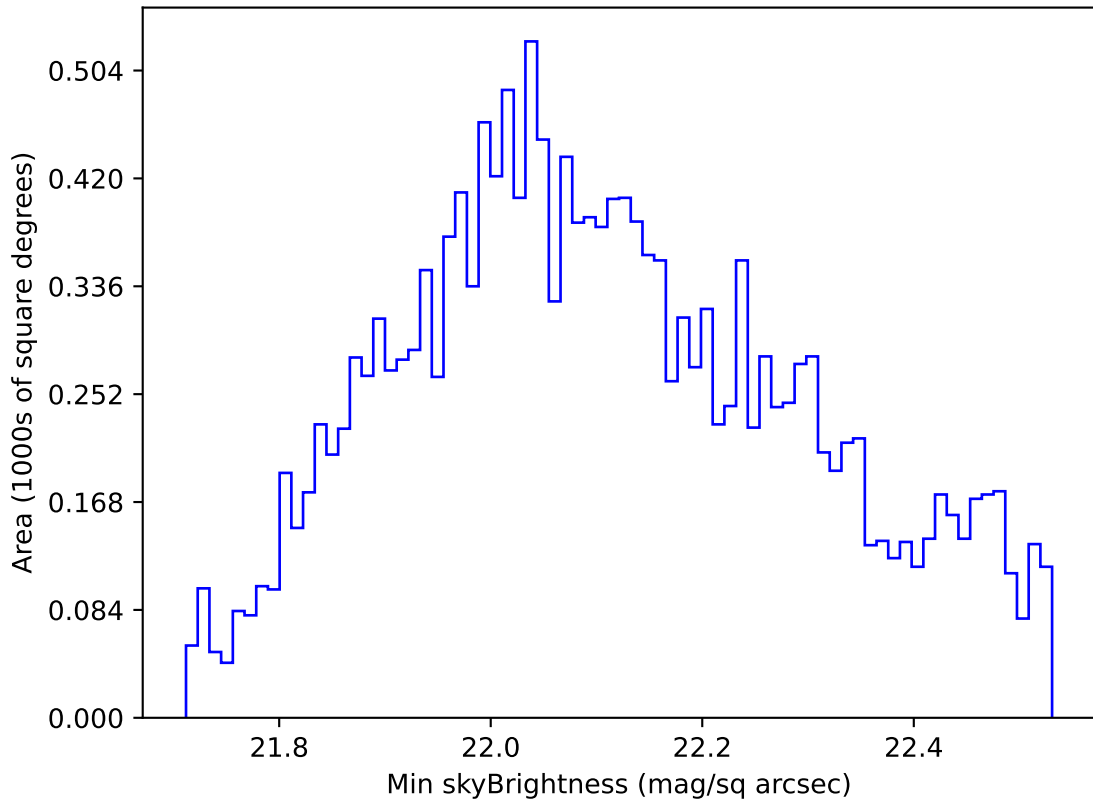
too_elab_r32_d2_griz_v3.4_10yrs WFD u band: Min skyBrightness
