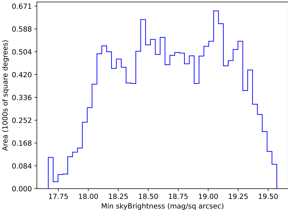
too_elab_r32_d2_griz_v3.4_10yrs WFD r band: Min skyBrightness
