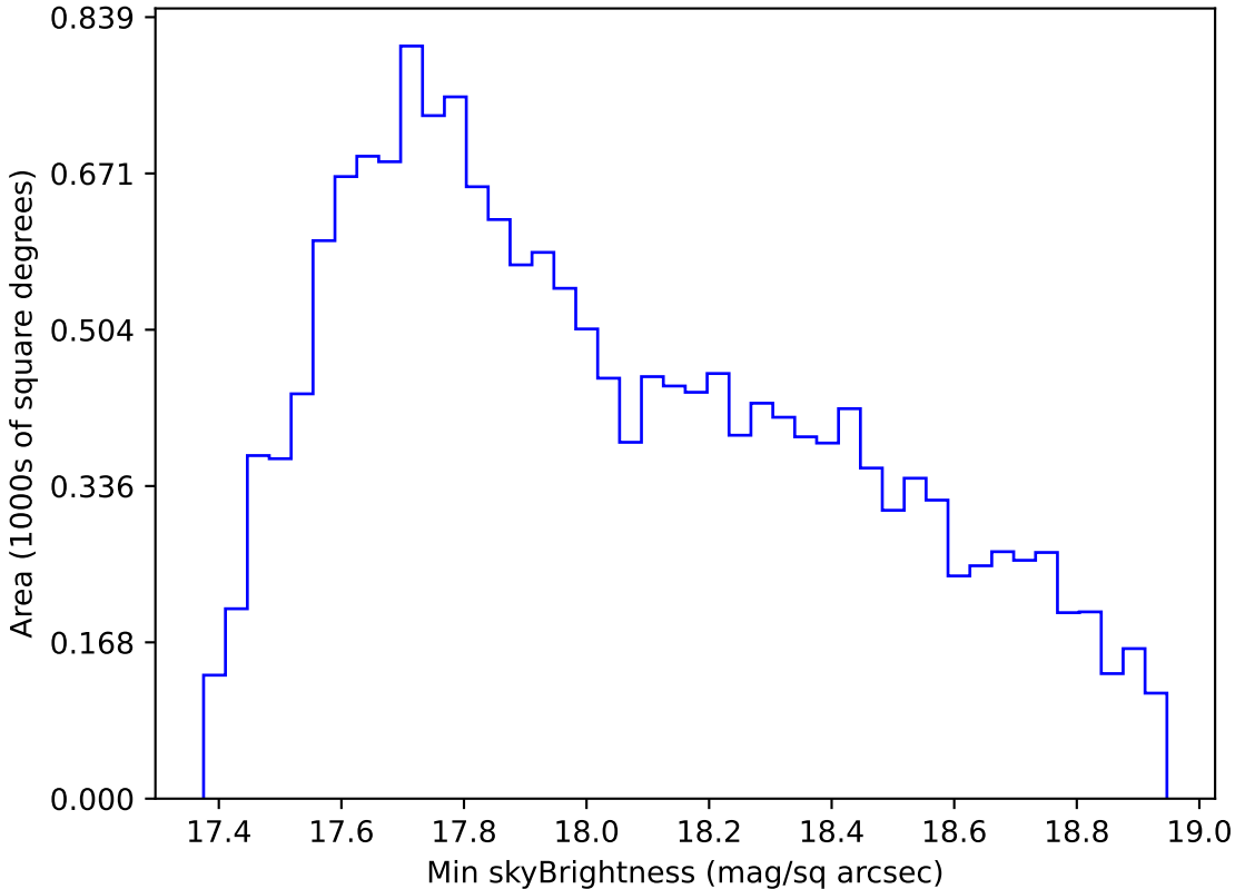
too_elab_r32_d2_griz_v3.4_10yrs WFD i band: Min skyBrightness
