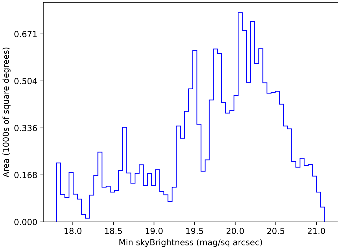
too_elab_r32_d2_griz_v3.4_10yrs WFD g band: Min skyBrightness
