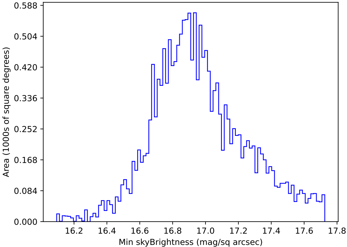
too_elab_r32_d2_griz_v3.4_10yrs WFD all bands: Min skyBrightness
