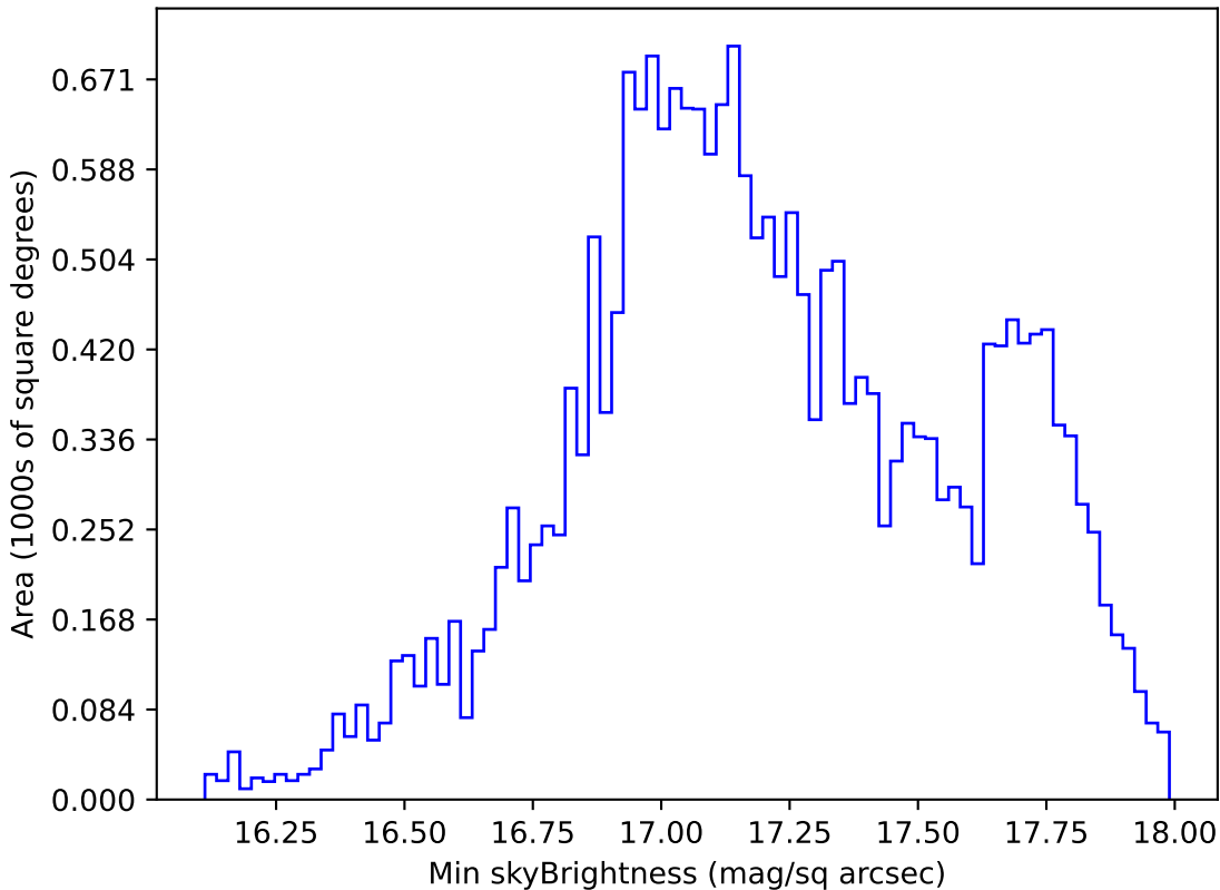
too_elab_r32_d2_griz_v3.4_10yrs All sky y band: Min skyBrightness
