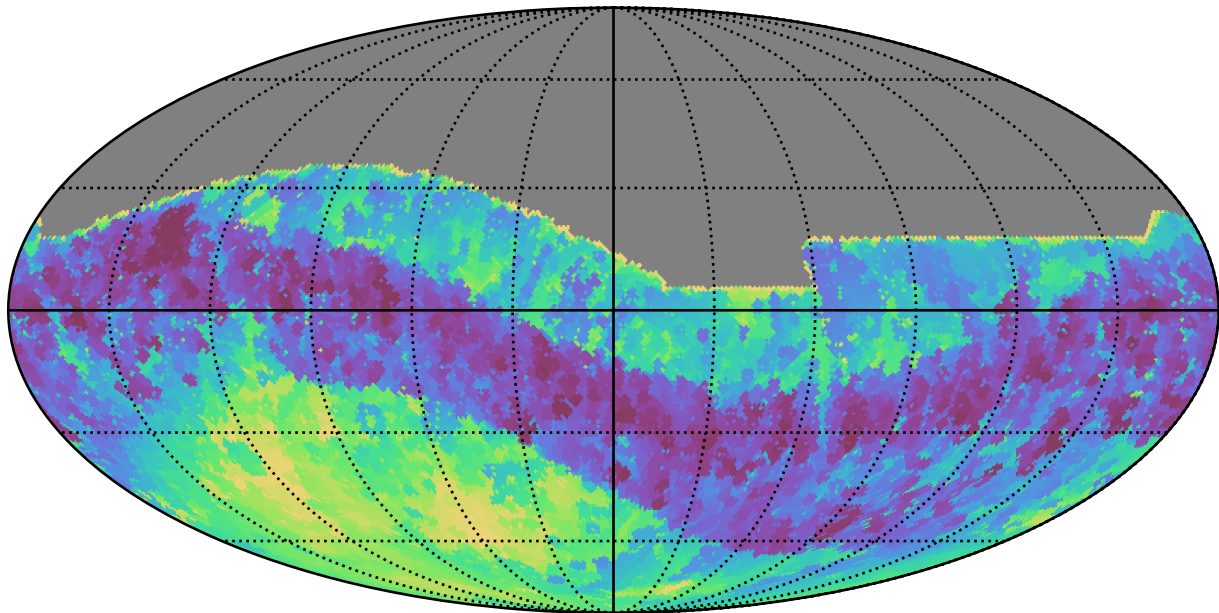
too_elab_r32_d2_griz_v3.4_10yrs All sky i band: Min skyBrightness
