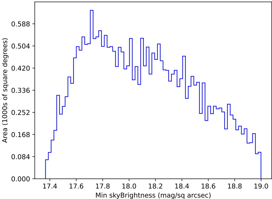
too_elab_r32_d2_griz_v3.4_10yrs All sky i band: Min skyBrightness
