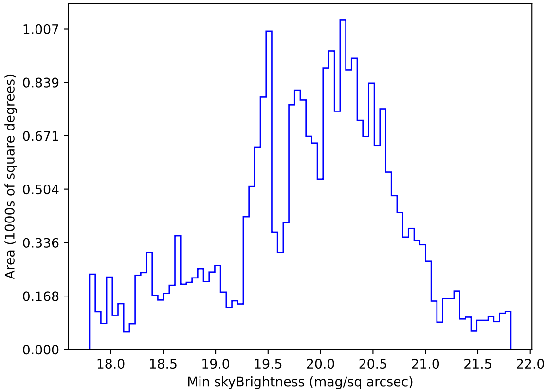
too_elab_r32_d2_griz_v3.4_10yrs All sky g band: Min skyBrightness
