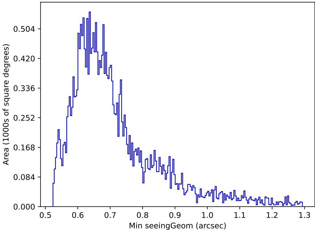
too_elab_r32_d2_griz_v3.4_10yrs Yr 1 g band: Min seeingGeom
