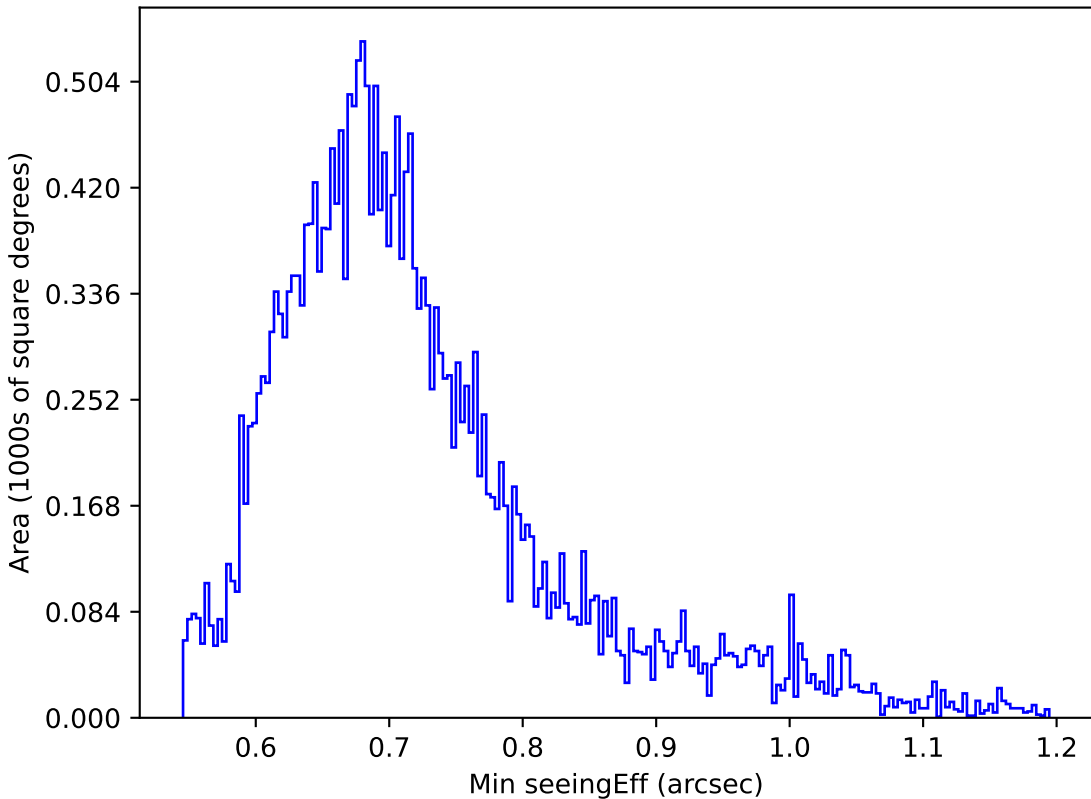
too_elab_r32_d2_griz_v3.4_10yrs Yr 1 z band: Min seeingEff
