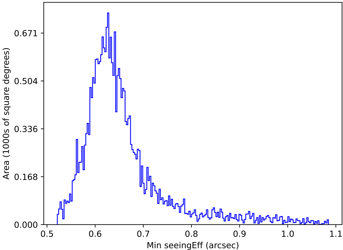
too_elab_r32_d2_griz_v3.4_10yrs Yr 1 all bands: Min seeingEff
