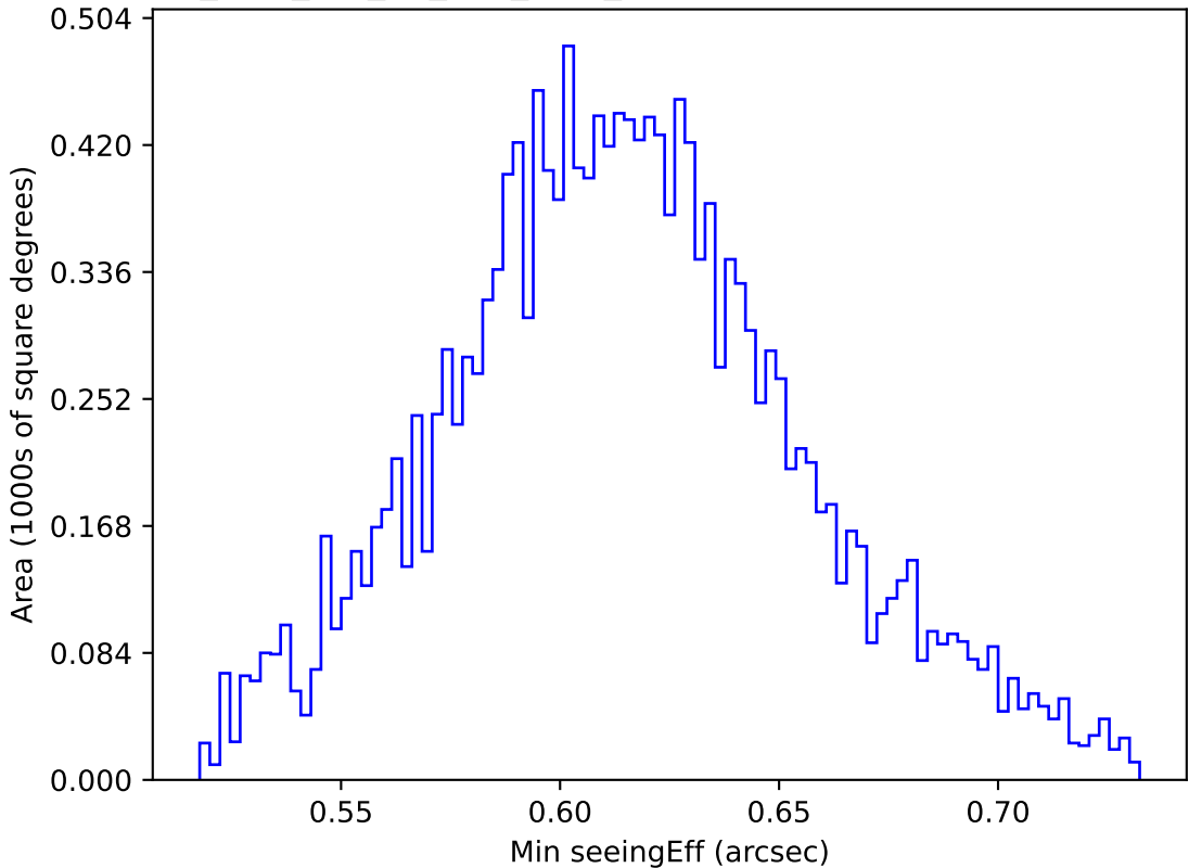
too_elab_r32_d2_griz_v3.4_10yrs WFD z band: Min seeingEff
