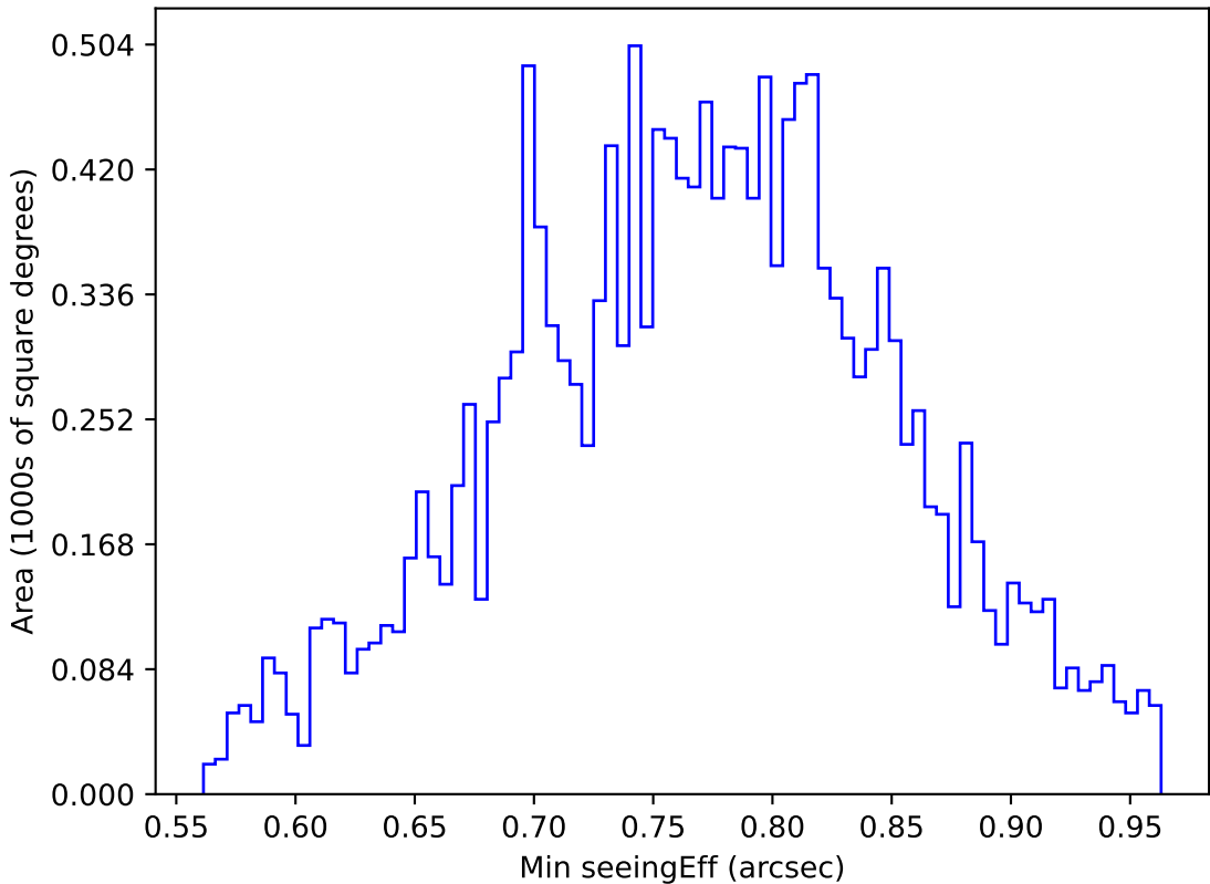
too_elab_r32_d2_griz_v3.4_10yrs WFD u band: Min seeingEff
