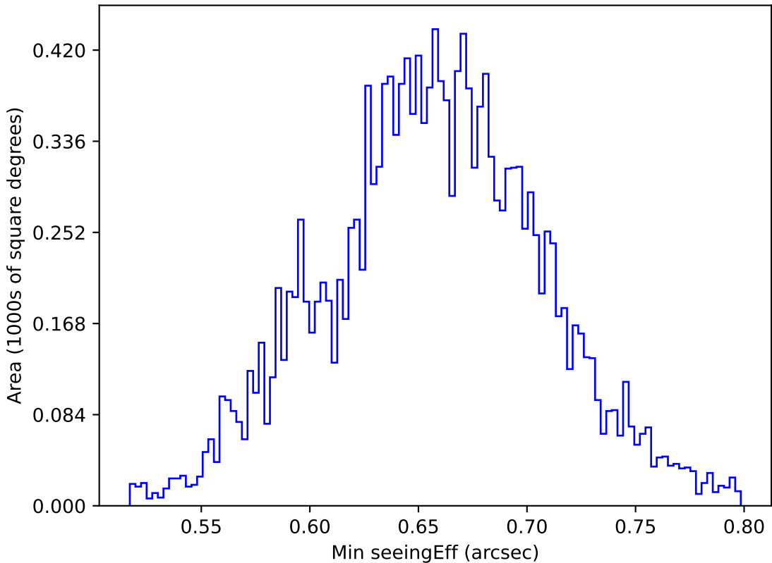
too_elab_r32_d2_griz_v3.4_10yrs WFD g band: Min seeingEff
