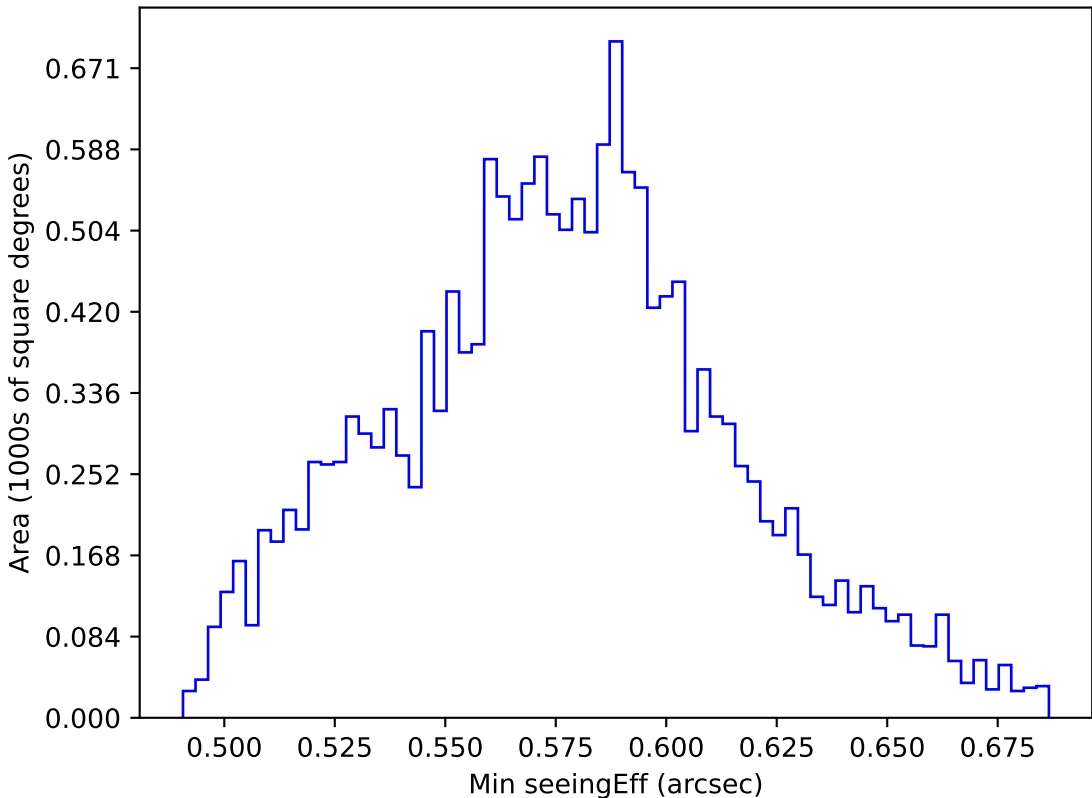
too_elab_r32_d2_griz_v3.4_10yrs WFD all bands: Min seeingEff
