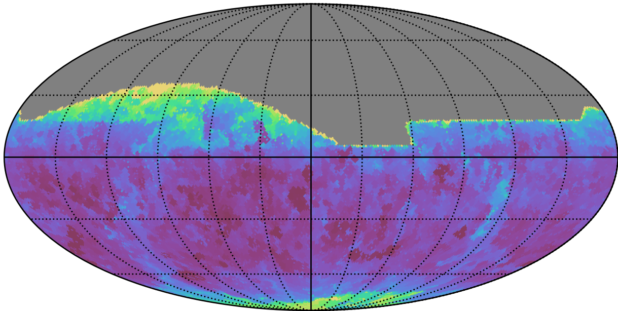
too_elab_r32_d2_griz_v3.4_10yrs All sky z band: Min seeingEff
