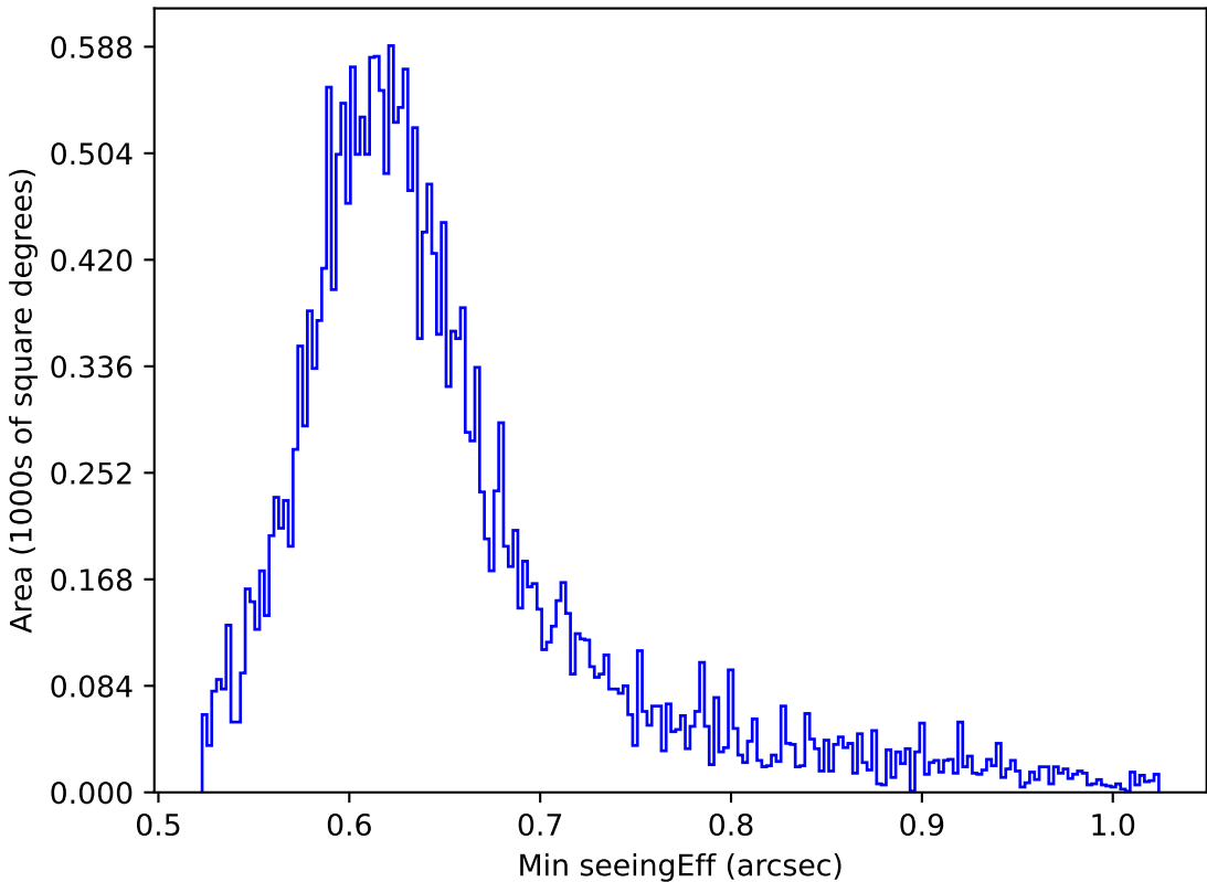
too_elab_r32_d2_griz_v3.4_10yrs All sky z band: Min seeingEff
