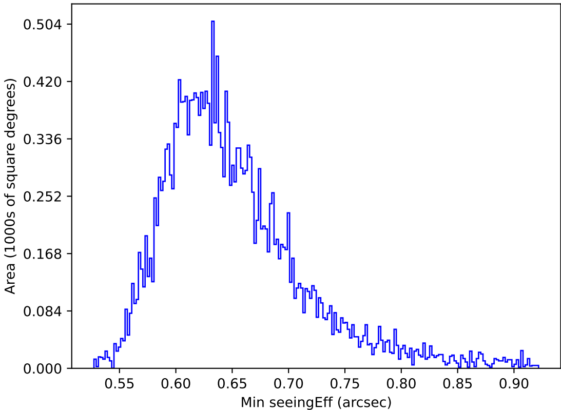
too_elab_r32_d2_griz_v3.4_10yrs All sky y band: Min seeingEff
