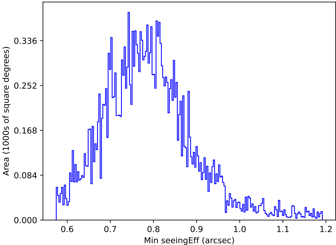
too_elab_r32_d2_griz_v3.4_10yrs All sky u band: Min seeingEff
