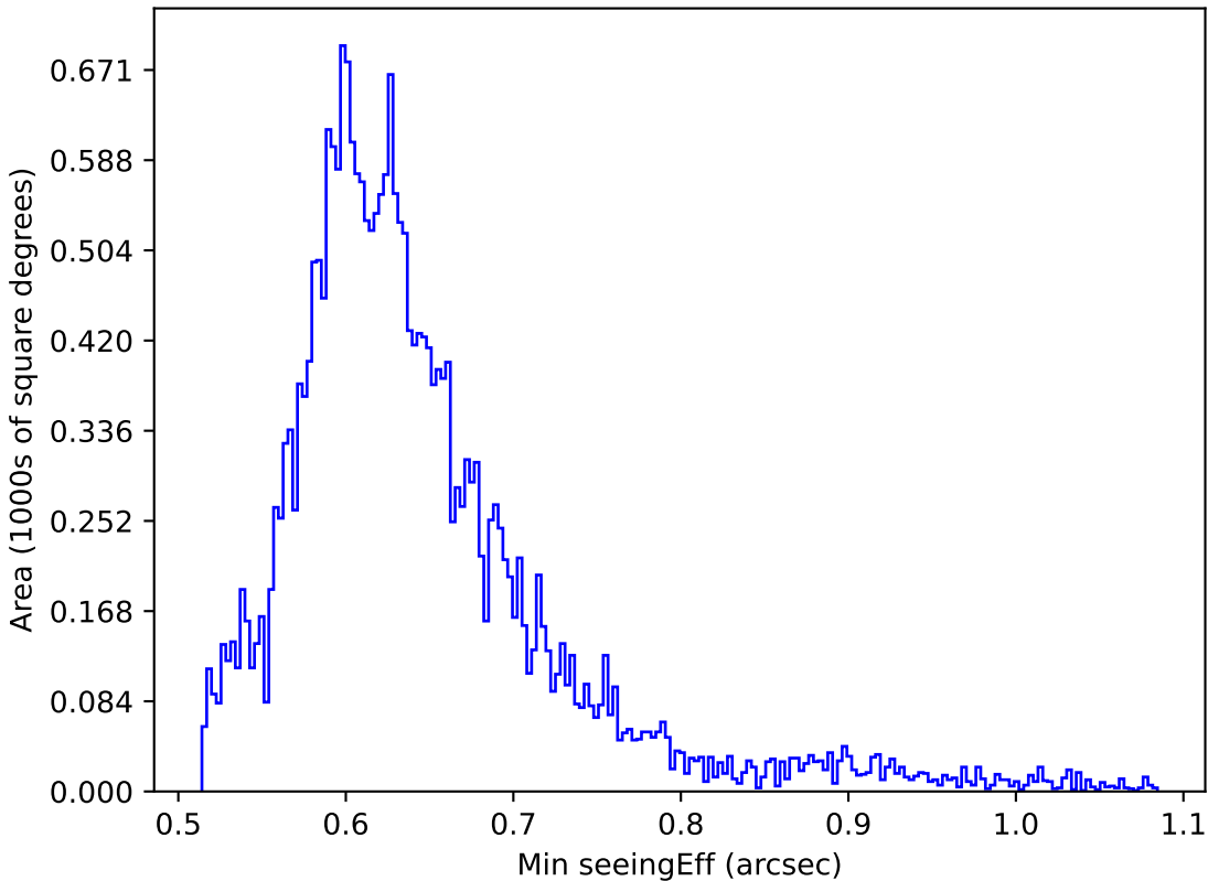
too_elab_r32_d2_griz_v3.4_10yrs All sky r band: Min seeingEff
