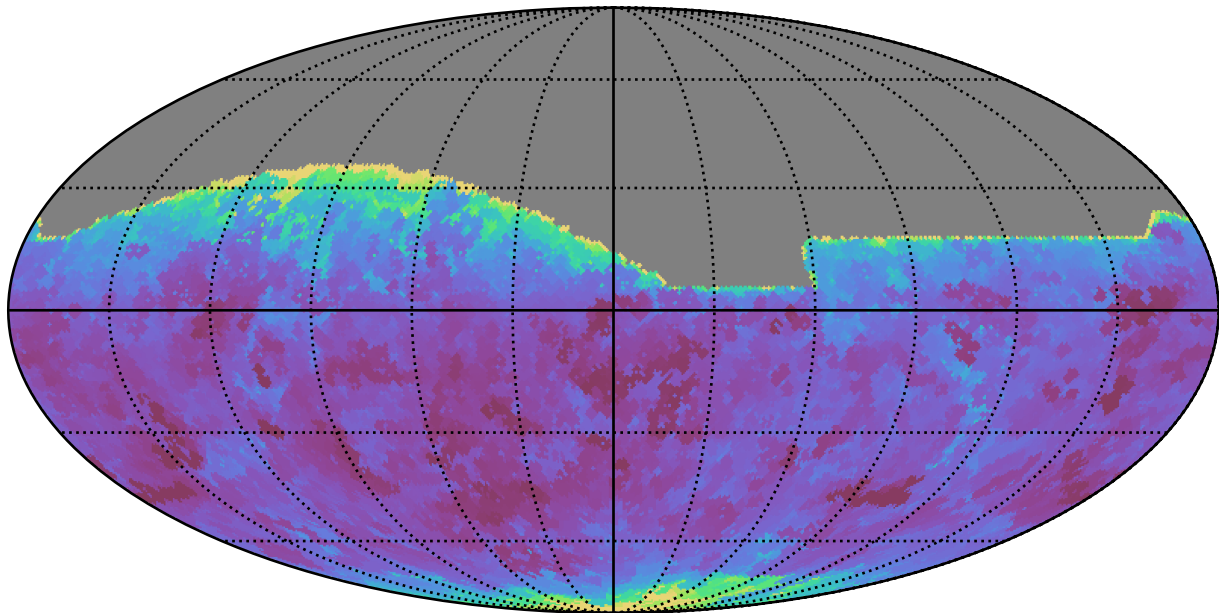
too_elab_r32_d2_griz_v3.4_10yrs All sky i band: Min seeingEff
