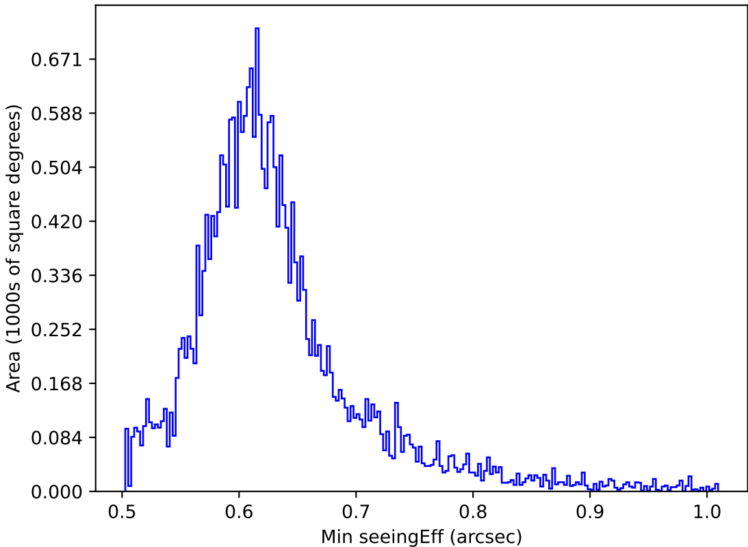
too_elab_r32_d2_griz_v3.4_10yrs All sky i band: Min seeingEff
