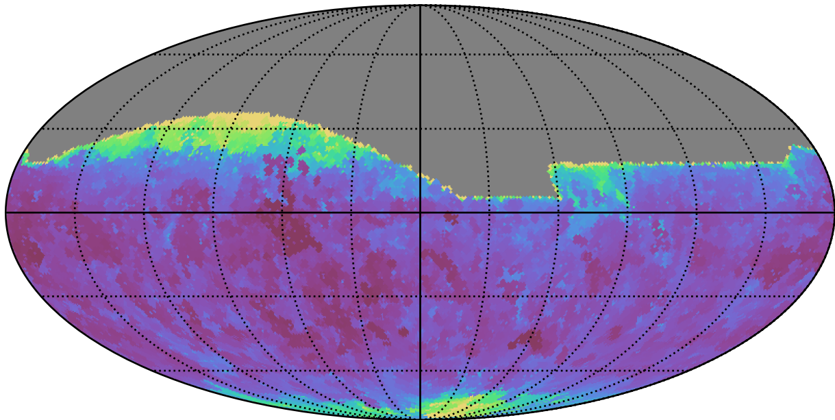
too_elab_r32_d2_griz_v3.4_10yrs All sky g band: Min seeingEff
