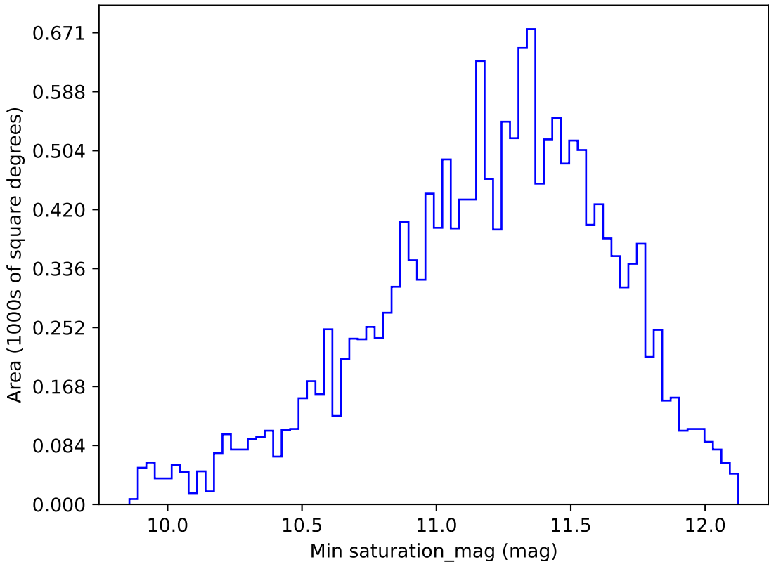
too_elab_r32_d2_griz_v3.4_10yrs WFD y band: Min saturation_mag
