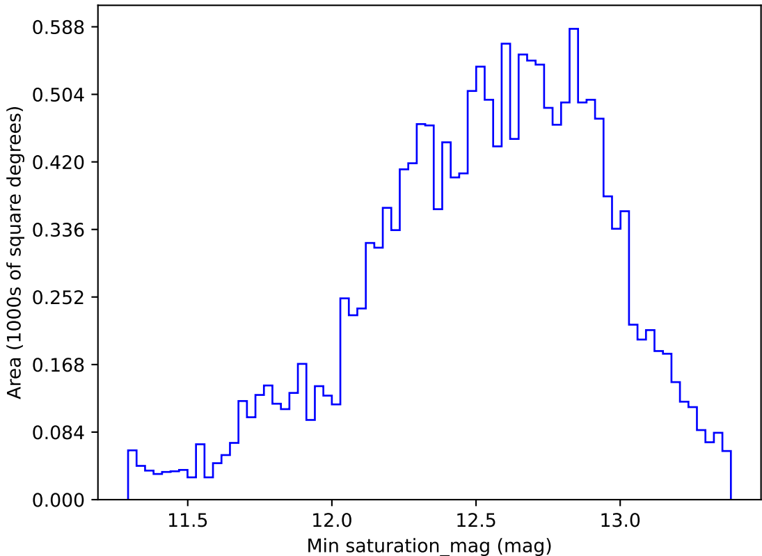
too_elab_r32_d2_griz_v3.4_10yrs WFD r band: Min saturation_mag
