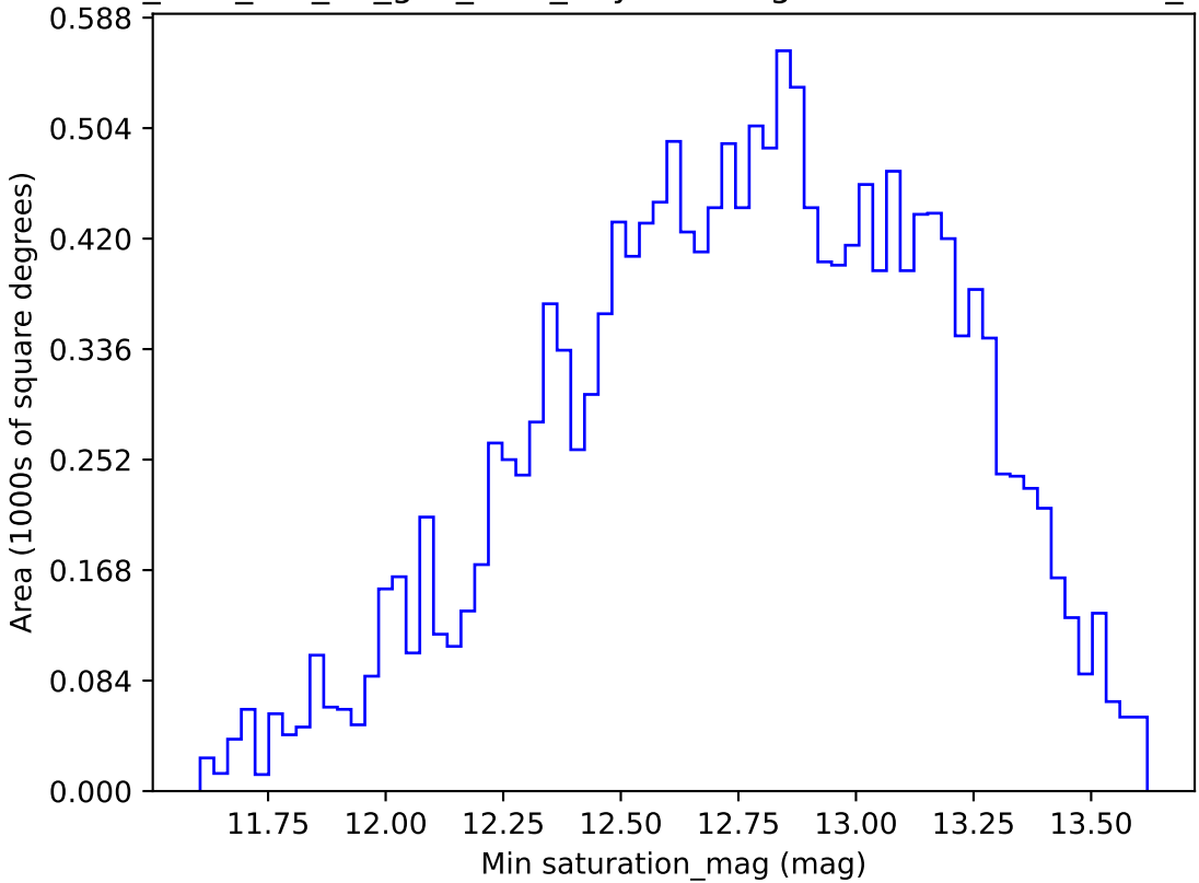
too_elab_r32_d2_griz_v3.4_10yrs WFD g band: Min saturation_mag
