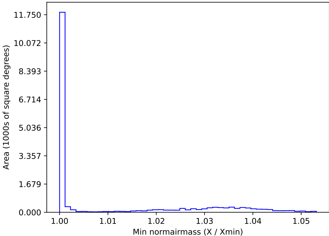
too_elab_r32_d2_griz_v3.4_10yrs WFD u band: Min normairmass
