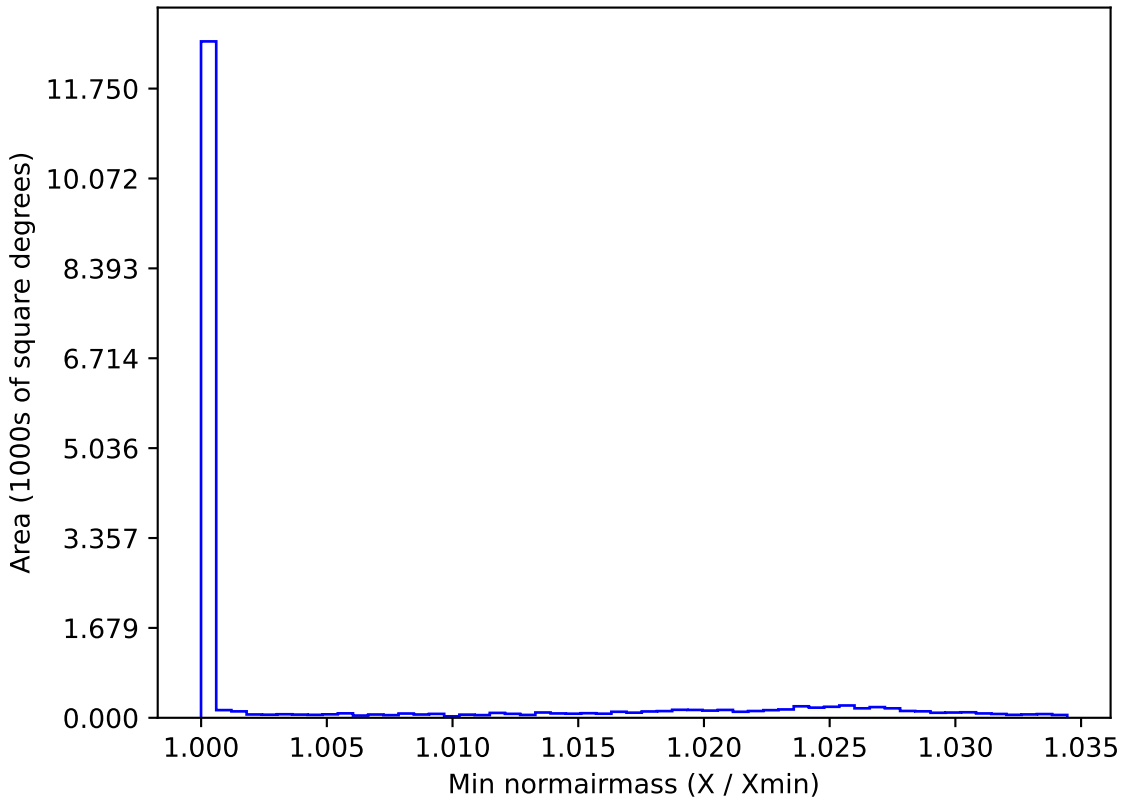
too_elab_r32_d2_griz_v3.4_10yrs WFD i band: Min normairmass
