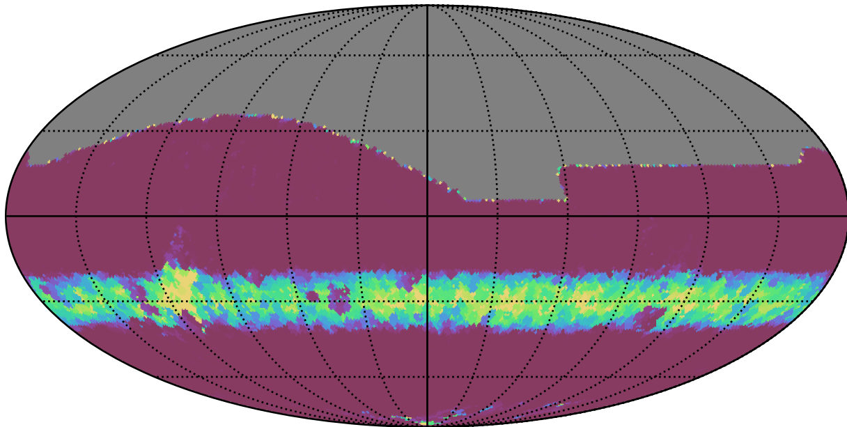
too_elab_r32_d2_griz_v3.4_10yrs All sky r band: Min normairmass
