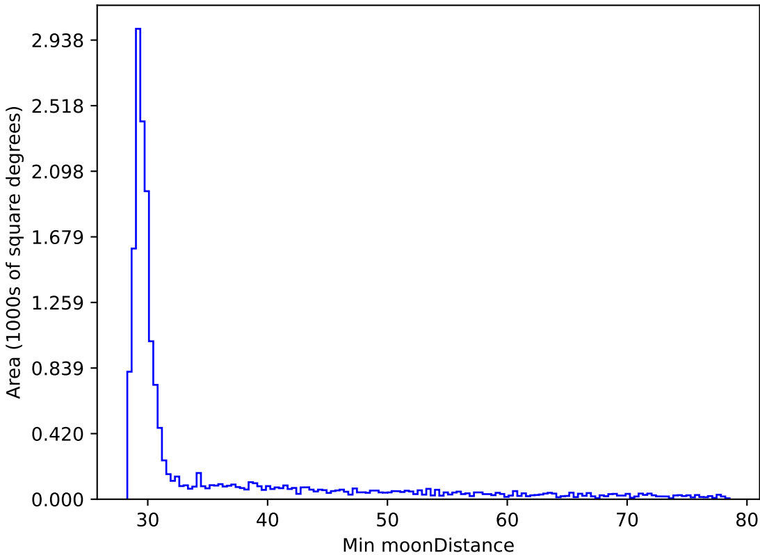
too_elab_r32_d2_griz_v3.4_10yrs WFD y band: Min moonDistance
