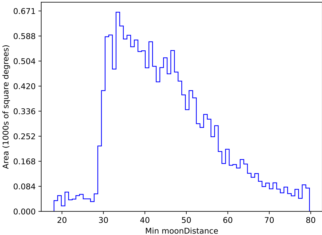
too_elab_r32_d2_griz_v3.4_10yrs WFD g band: Min moonDistance
