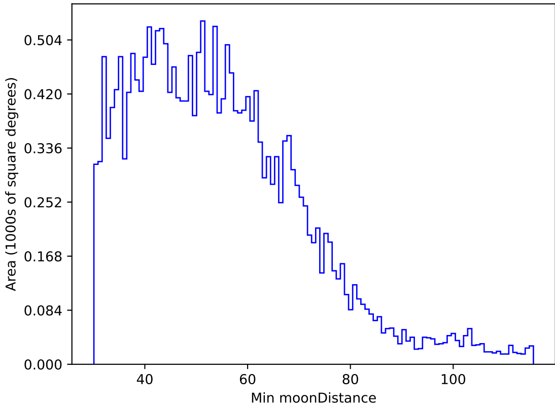
too_elab_r32_d2_griz_v3.4_10yrs All sky u band: Min moonDistance
