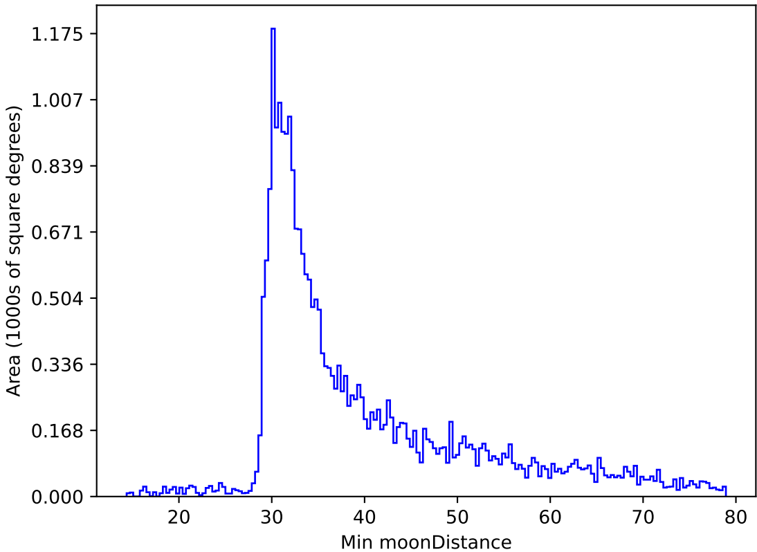
too_elab_r32_d2_griz_v3.4_10yrs All sky r band: Min moonDistance
